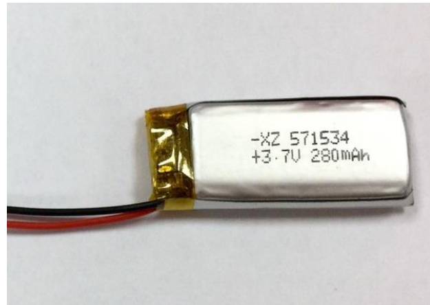
XZ571534 3.7V 280mAh
